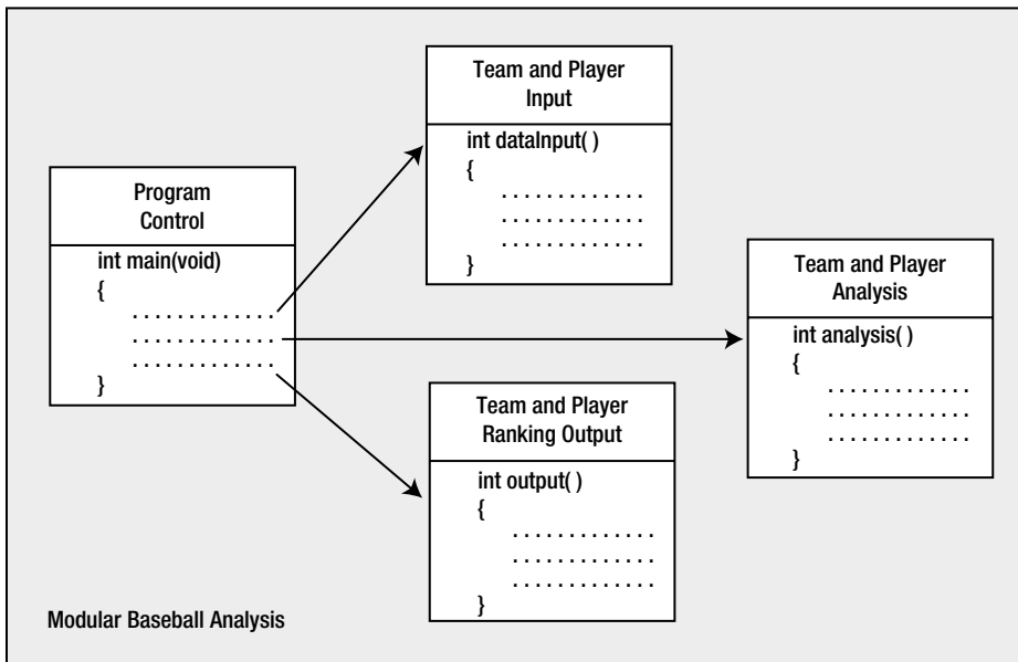
Figure 1-3. Modular programming
